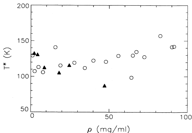
FIG. 5. The extrapolated temperature ( T^* ) as obtained in Fig. 4 is shown as a function of concentration for TMV in 25 mM phosphate (O) and in unbuffered water (▲). The samples of highest concentration for each data set are in coexistence with the nematic phase. T^* = 120 \pm 20 K independent of concentration and ionic strength.
