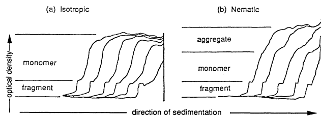
FIG. 13. Ultraviolet absorbance scans through sedimenting samples of material taken from coexisting isotropic and nematic phases of the U2 5 mM fragmented sample (same as in Figs. 10 and 11). The traces in (a) are from material taken from the isotropic phase and in (b) the material is from the nematic phase. The ordinate (optical density at 280 nm) is proportional to the total material in the cell and the abscissa is proportional to the distance perpendicular from the centrifuge rotation axis. Scans from left to right are at progressively later times, and show the material sedimenting towards the bottom of the cell. Each step in a scan is caused by a species of material that sediments at different rates. The position of each step is as a function of time is used to determine the Svedburg constant and is related to the length of the particles through Eqs. (25)–(27) and summarized in Fig. 12. The height of each step is proportional to the weight concentration of each species. The measured Svedburg constant and weight percentage of the species are presented in Table IV. In the isotropic phase (a) two steps are seen, corresponding to a lighter fragment and heavier monomer. In the nematic phase (b) three steps are observed, the fragments and monomer fractions as in the isotropic phase and additionally a heavier aggregate, which has preferentially segregated to the nematic phase.
